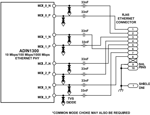
Figure 40. Media Dependent Interface Using Capacitive Coupling
