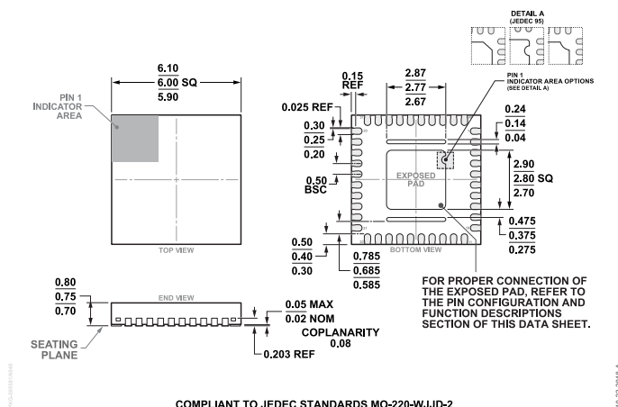
Figure 47. 40-Lead Lead Frame Chip Scale Package [LFCSP] 6 mm x 6 mm Body and 0.75 mm Package Height (CP-40-26) Dimensions shown in millimeters
