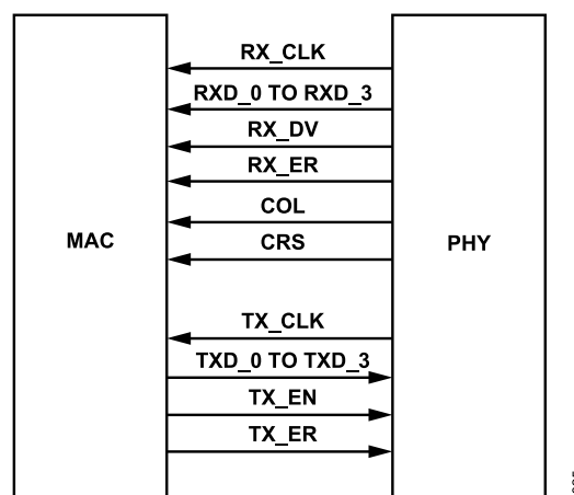
Figure 23. MII MAC to PHY Interface Signals
