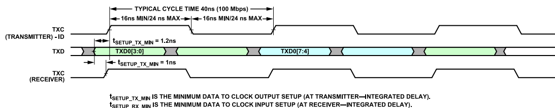
Figure 36. RGMII Timing Example for 100 Mbps Data Rate, with Internal Delay Enabled
