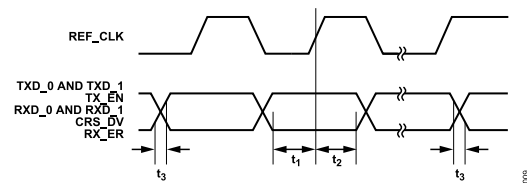
Figure 9. RMII Timing
