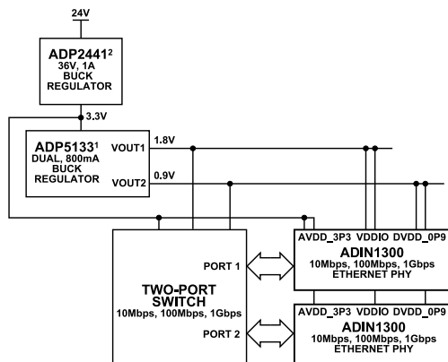
Figure 42. Recommended Power Solution with 24 V System Power, Where RGMI is Operating at VDDIO = 1.8 V
